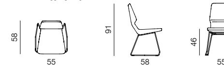
CHAIR SLED BASE dimensions 55 x 58 x 91 cm
