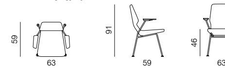
CHAIR METAL dimensions 63 x 59 x 91 cm
