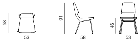
CHAIR SLED METAL LEGS dimensions 53 x 58 x 91 cm
