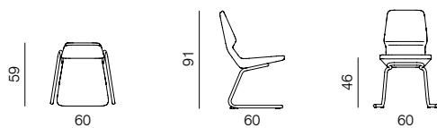
CHAIR CANTILEVER dimensions 60 x 59 x 91 cm
