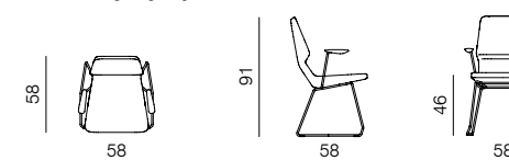
CHAIR SLED BASE WITH ARMRESTS dimensions 58 x 58 x 91 cm
