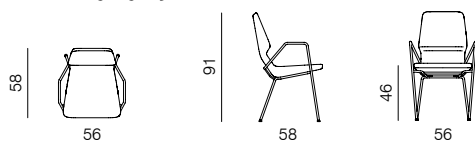
CHAIR SLED METAL LEGS WITH ARMRESTS dimensions 56 x 58 x 91 cm
