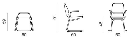
CHAIR CANTILEVER WITH ARMRESTS dimensions 60 x 59 x 91 cm
